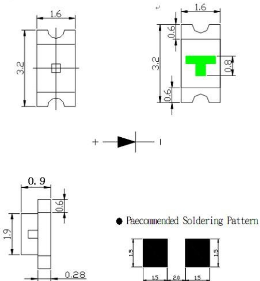
Package Outline Dimensions:
